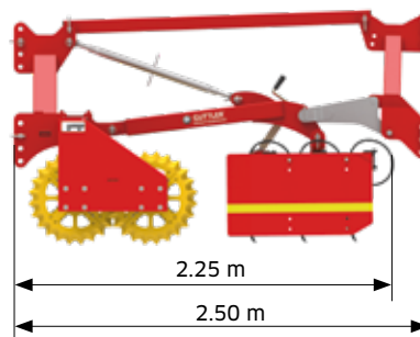
Headstock for rear linkage
