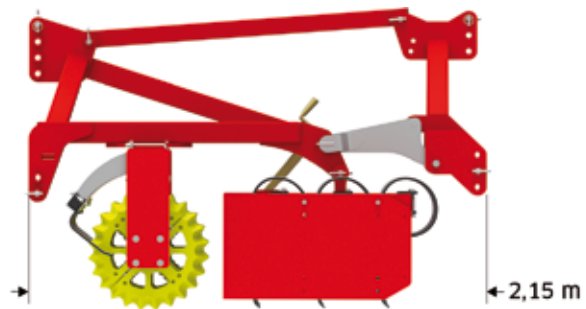
Front press with headstock for rear linkage
